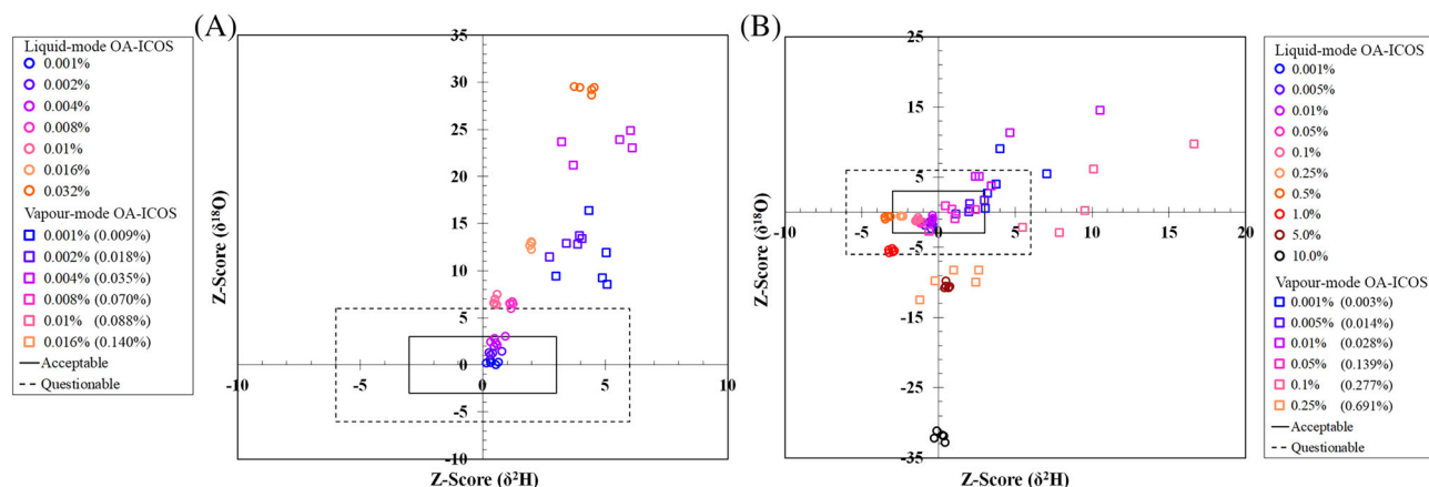
FIGURE 2 Z-score plots for (A) methanol-contaminated and (B) ethanol-contaminated samples analysed by vapour and liquid modes. A Z-score of <|3| (falling within the solid box) is considered acceptable, |3-6| (falling within the dashed box) is questionable, and >|6| (falling outside of the dashed box) is unacceptable. Vapour-mode results for methanol concentrations >0.016\% and ethanol concentrations >0.25\% are not included due to negative absorbance issues. Liquid-mode Z-scores for methanol concentrations >0.032\% are not shown as the scores become so large as to obscure the plot. Concentrations in parentheses for vapour-mode data are the vapour-phase concentrations of contaminants in the analysis headspace
